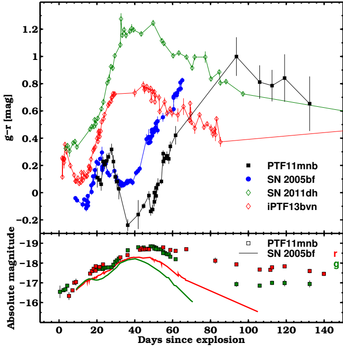
Fig. 3. Top panel: color comparison of g - r between PTF11mnb, SN 2005bf, SN Ib iPTF13bvn (Fremling et al. 2016), and SN Iib 2011dh (Ergon et al. 2014, 2015). The first two SNe reach a red peak in the color, which coincides with the early peak in their light curves (see bottom panel ). Then their g - r becomes bluer reaching a minimum when the main peak of the light curves occurs. Thereafter, they rapidly evolve to redder colors. PTF11mnb also shows a shallow trend to the blue after \sim 100 d, when the light curves are flatter (see bottom panel ) and when SN 2005bf was not observed. iPTF13bvn and SN 2011dh evolve very differently, reaching a g - r minimum at peak magnitude, followed by a linear trend to the red and a final flatter color after \sim 30 d. Bottom panel: absolute g - and r -band light curves of PTF11mnb and SN 2005bf, plotted as a reference for the various phases of the color evolution.
