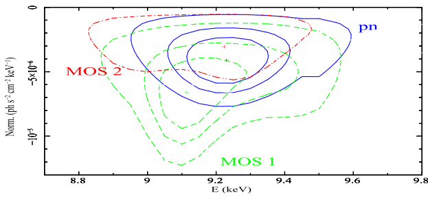
Fig. 4. Confidence contours plot of the Gaussian absorption line normalization vs. its rest-frame energy for each single EPIC instrument. Contours confidence levels are as in Fig. 2.
