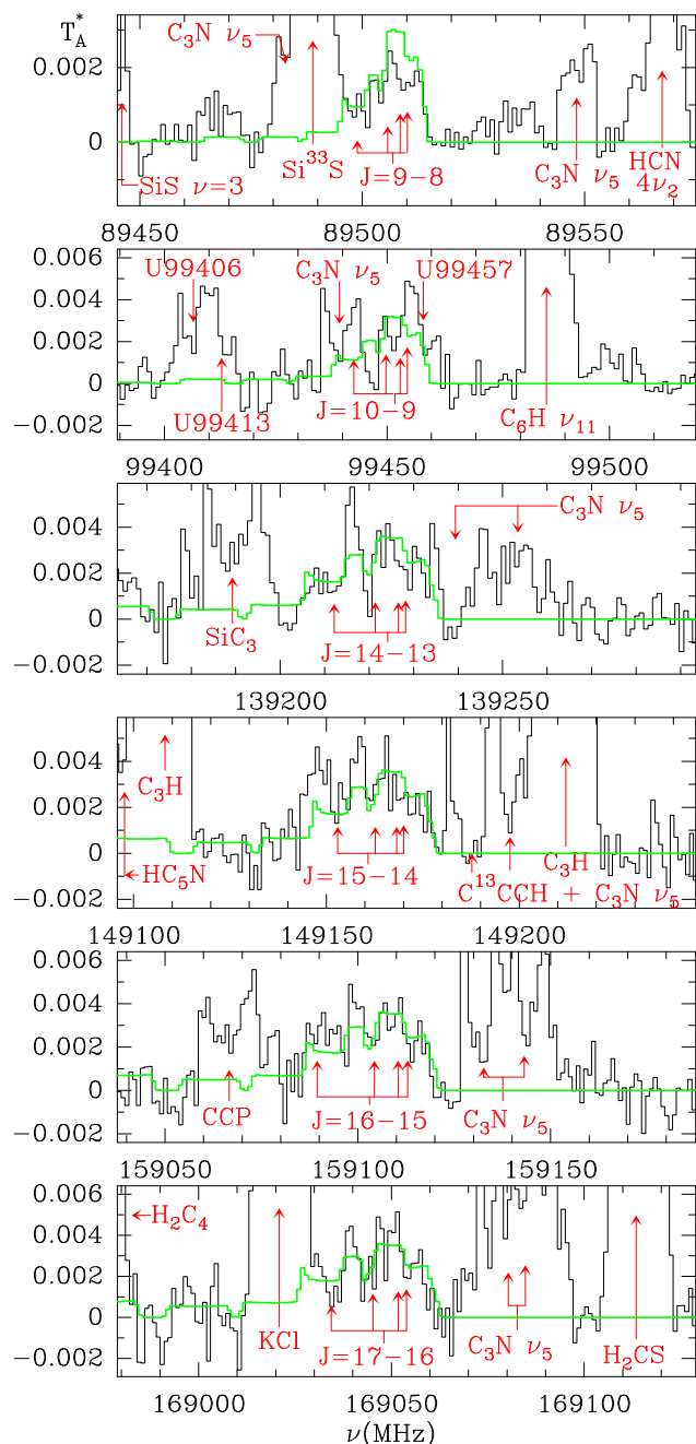
Fig. A.1. Observed rotational lines of silyl cyanide, \text{SiH}_3\text{CN} , toward IRC+10216. Spectral resolution is 1 MHz and the intensity scale is antenna temperature. Rest frequencies are indicated for an assumed LSR velocity of the source of -26.5 km \text{s}^{-1} . The arrows indicate the position of the K = 0, 1, 2, and 3 components of each J \rightarrow (J-1) rotational transition. The identification of other features found in the spectra is indicated. Green lines correspond to the emerging line profiles calculated with the model discussed in the text.
